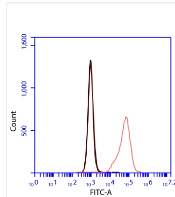
Flow Cytometry—Anti-SFXN1 Antibody (M25021)
