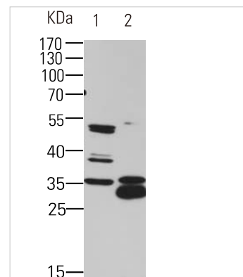
IP-Anti-SFXN1 Antibody(M25021)
