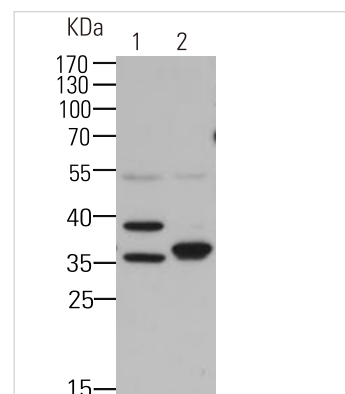
WB-Anti-SFXN1 Antibody(M25021)
