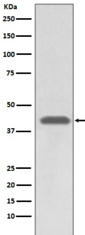
Western blot analysis of MHC class 1 expression in A549 cell lysate.
