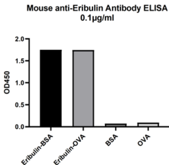
Fig1: ELISA Binding Assay of Anti-Eribulin Antibody to different proteins. ELISA analysis of Anti-Eribulin Monoclonal Antibody with Eribulin-BSA, Eribulin-OVA , BAS and OVA. Anti-Eribulin Monoclonal Antibody can bind to Eribulin-BSA or Eribulin-OVA but not carrier proteins.
